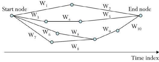
Fig. 2. An example of a lattice.
