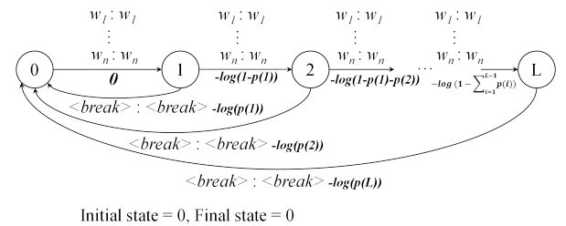
Figure 4: Sentence length model
