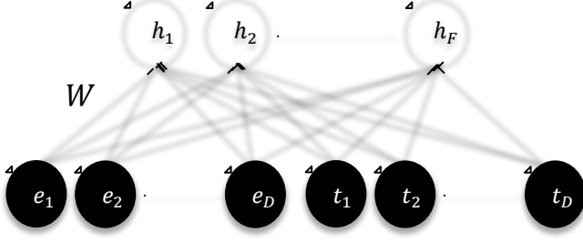
Figure 3: Restricted Boltzmann machine with 2 \times D visible units \mathbf{e} = \{e_1, e_2 \dots e_D\} for speaker enrolment utterance (left), \mathbf{t} = \{t_1, t_2 \dots t_D\} for test utterance (right) and F hidden units \mathbf{h} = \{h_1, h_2 \dots h_F\} .
